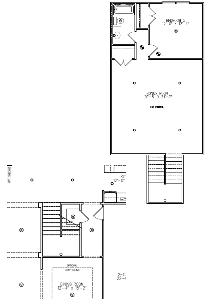
OAKLEIGH WITH BONUS STAIR LAYOUT
