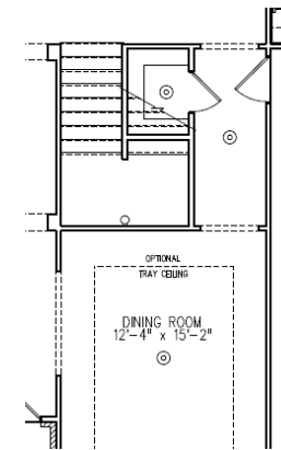
OAKLEIGH WITH BONUS STAIR LAYOUT
